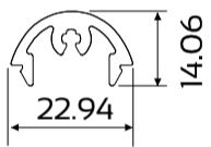
DIE No. W28819 Heavy Duty Handle Cap
