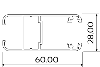
DIE No. W50855 Sash Frame
