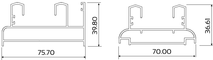
DIE No. W54272 Outer Frame with Lip
