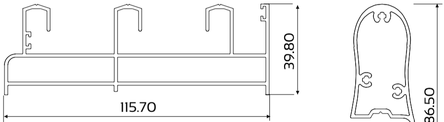
DIE No. W54299 Triple Frame with Lip
