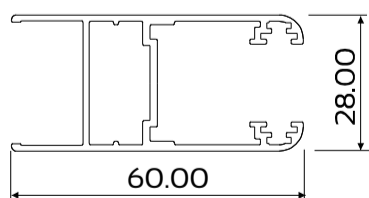
DIE No. W54274 Heavy Duty Sash Frame
