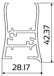
DIE No. W54022 Heavy Duty Handle
