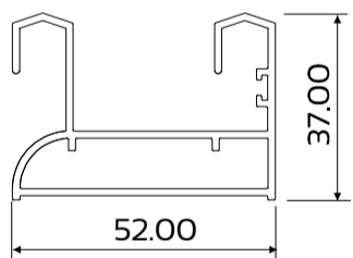
DIE No. W50827 Outer Frame Double Track
