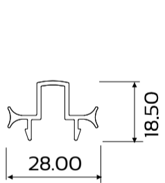
DIE No. W72183 Astragal for Meeting Stile
