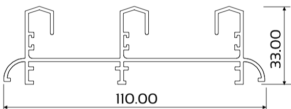
DIE No. W29233 Frame 44mm Flat
